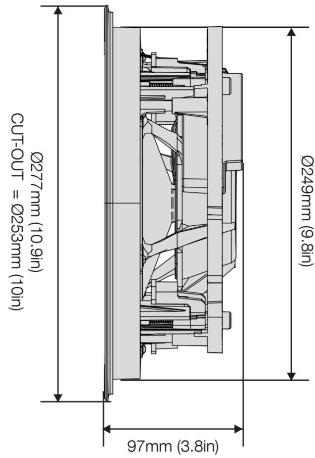
SIDE GRILLE OFF
